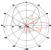
Radiation Pattern
